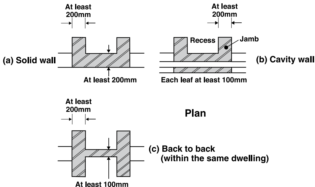
Diagram 28 Fireplace recesses
