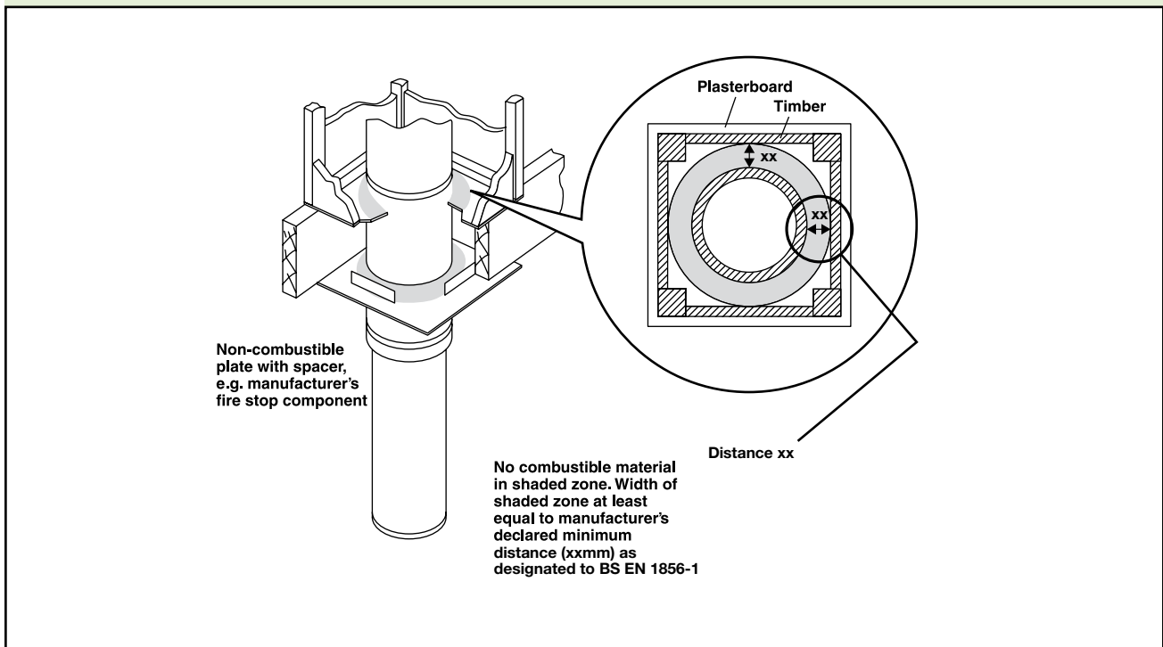
Diagram 13 The separation of combustibile material from a factory-made metal chimney designated to BS EN 1856-1:2003
