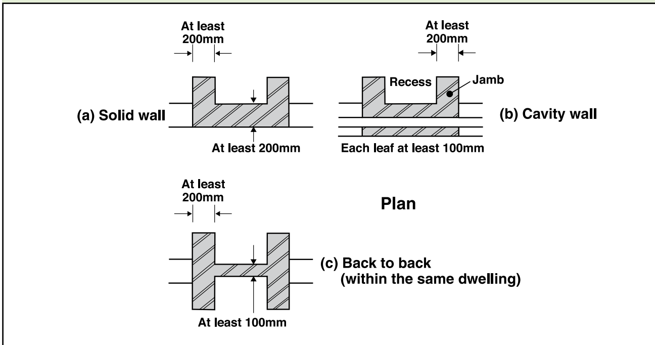
Diagram 28 Fireplace recesses
